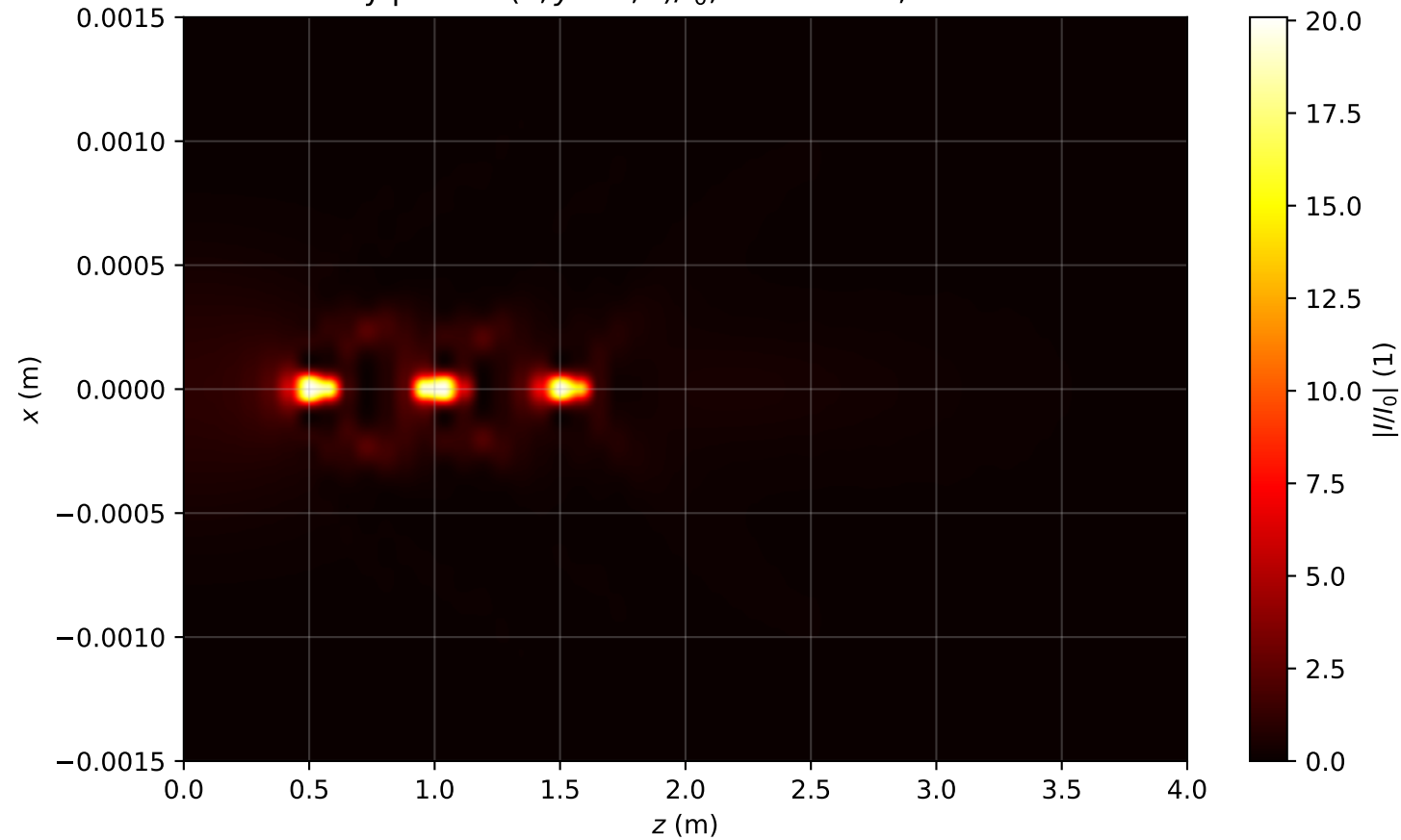
Intensity profile I(x, y = 0, z)/I_0 , P_{in}=5.5P_{cr} , artificial time
